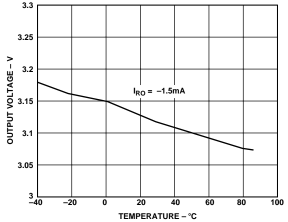
Figure 17. Receiver Output High Voltage vs. Temperature
