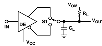
Figure 7. Driver Propagation Delay Test Circuit
